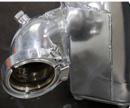
Direct-fit integration with Toyota LC HZJ79
