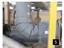
PHOTOS 1-5 Atlas Copco PV275 turbo, engine pipe, muffler and tailpipe blankets. Manifold blankets available (not pictured).
